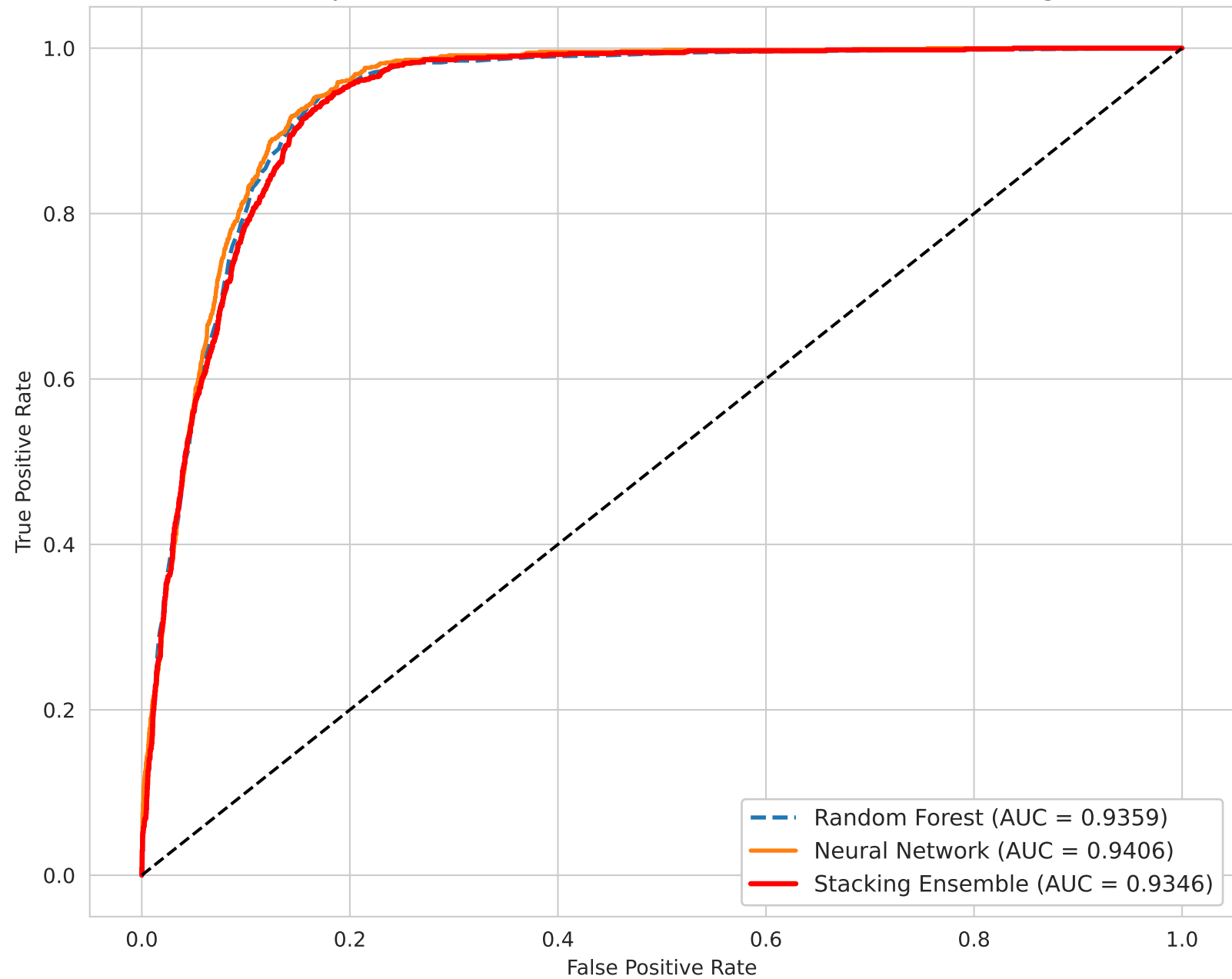
Comparison of ROC Curves: Baseline vs DL vs Stacking
