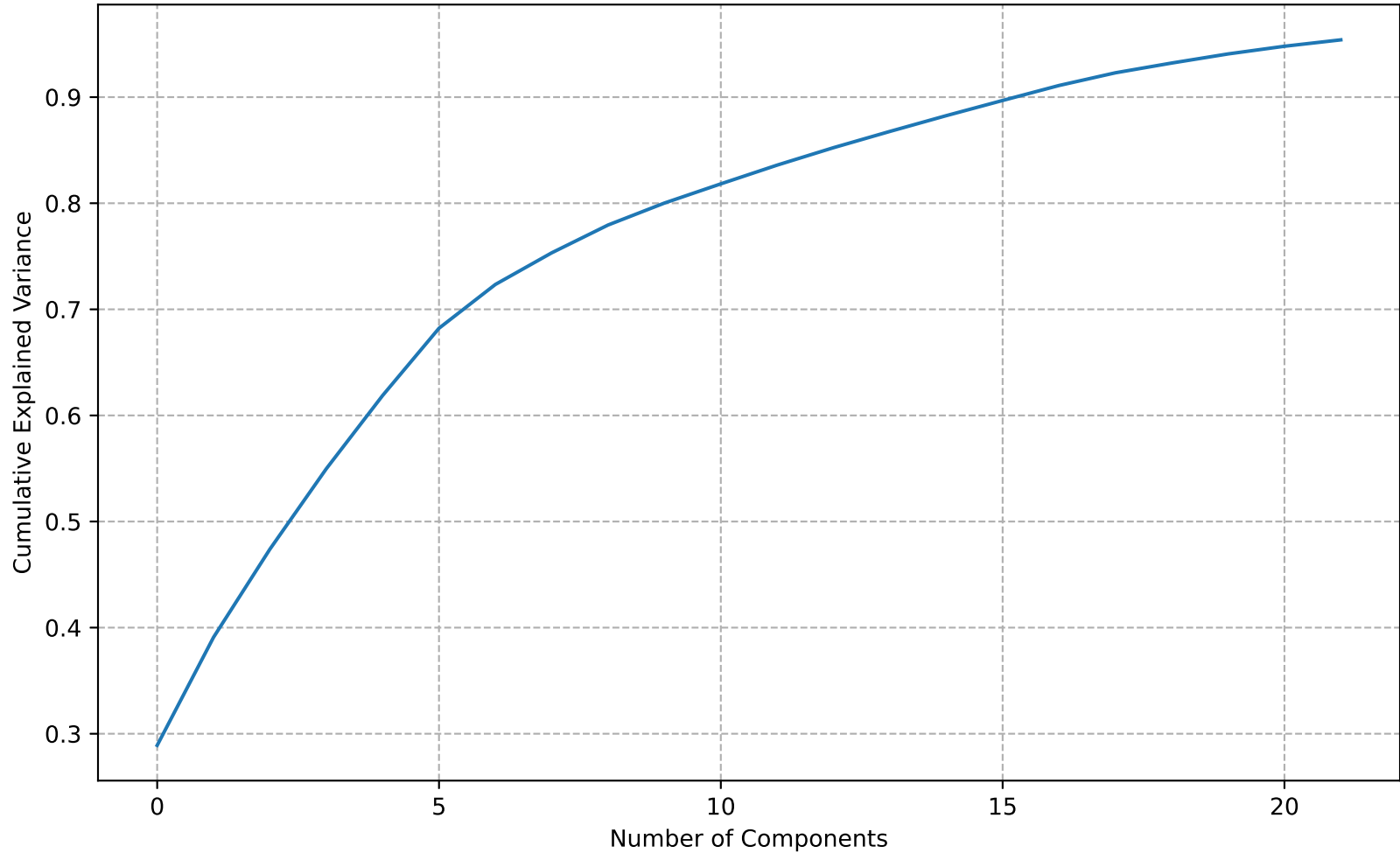
Explained Variance Plot for PCA
