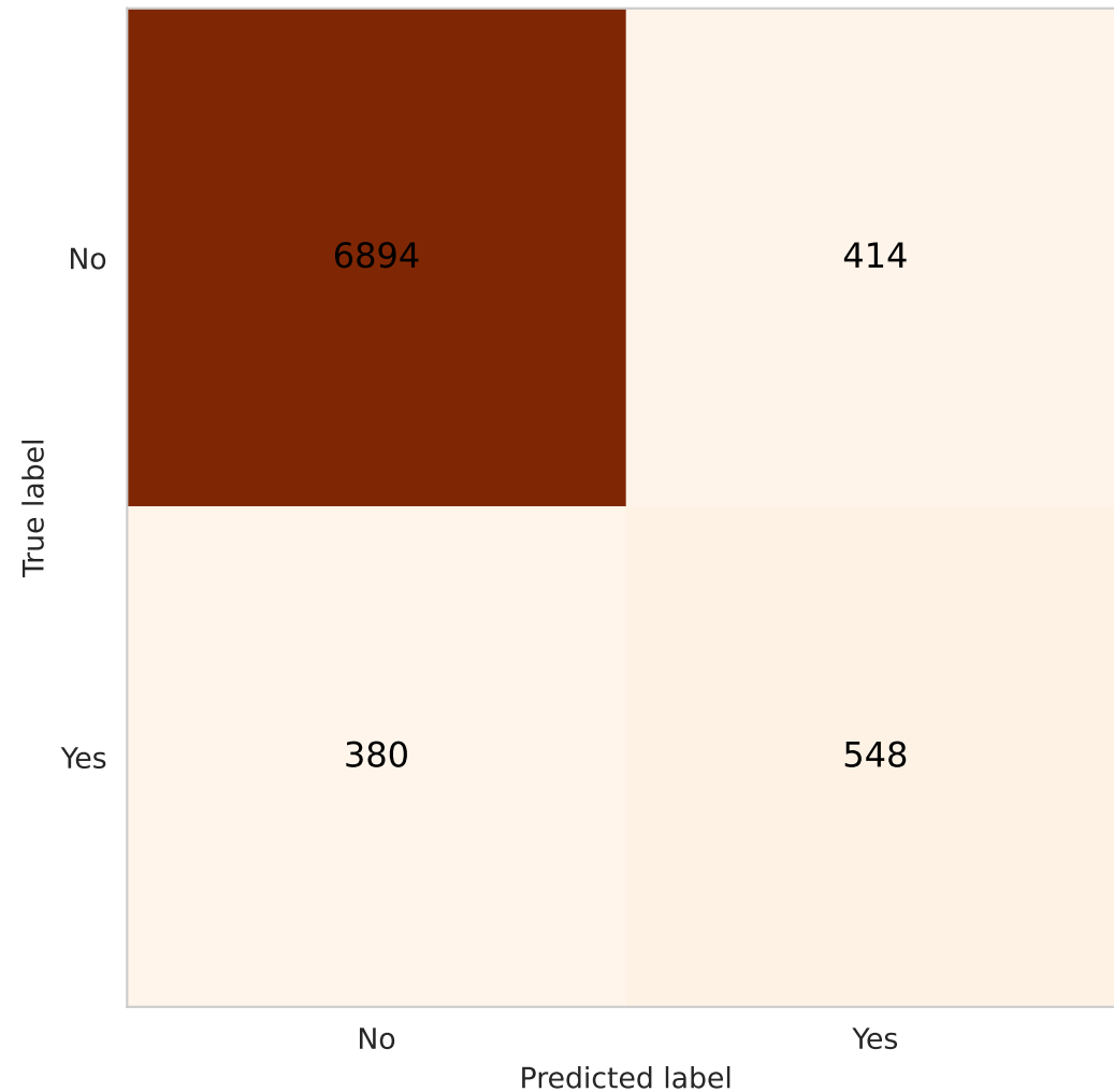
Stacking Ensemble (Greater Sensitivity / More Clients)
