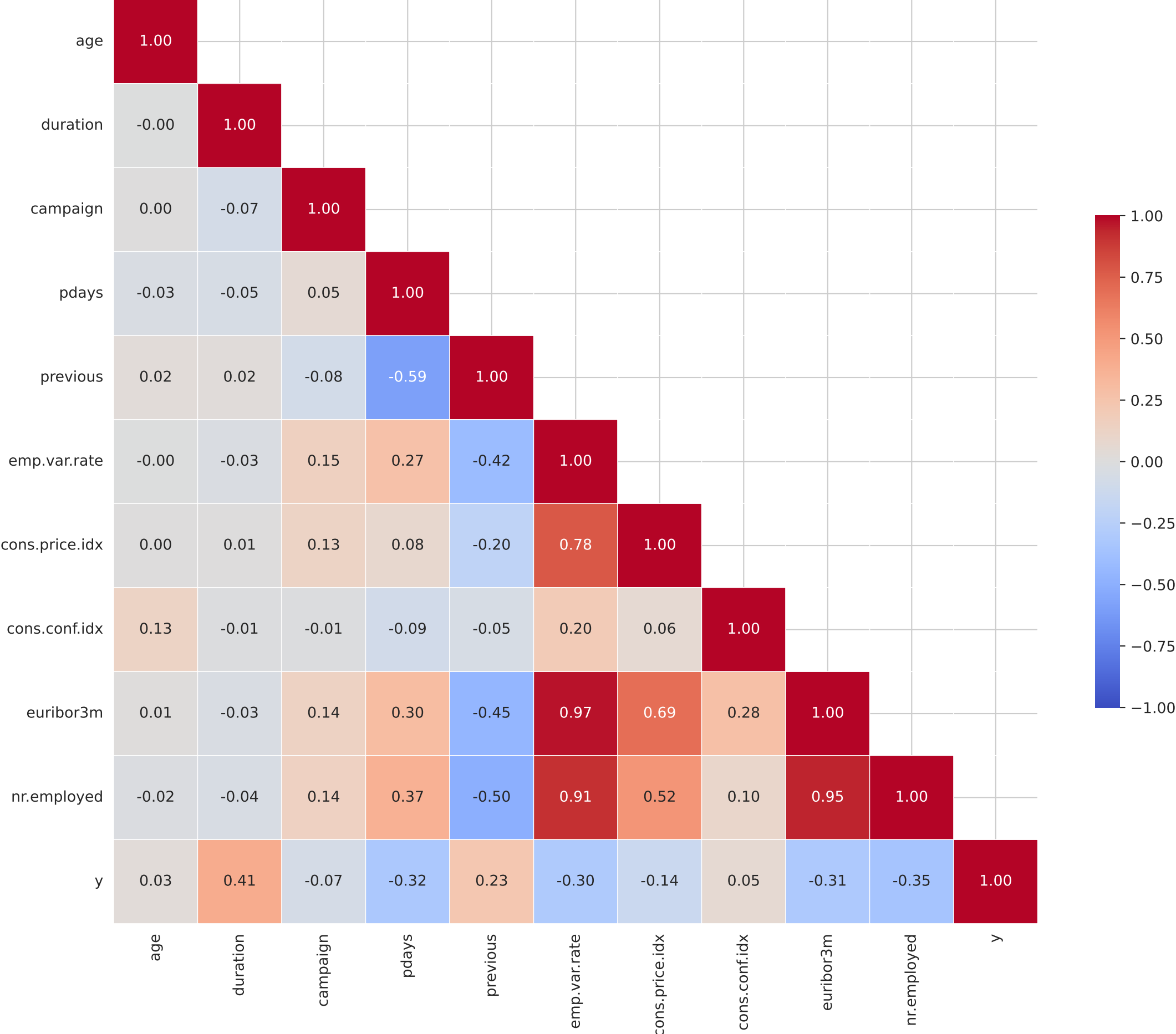
Correlation Matrix
