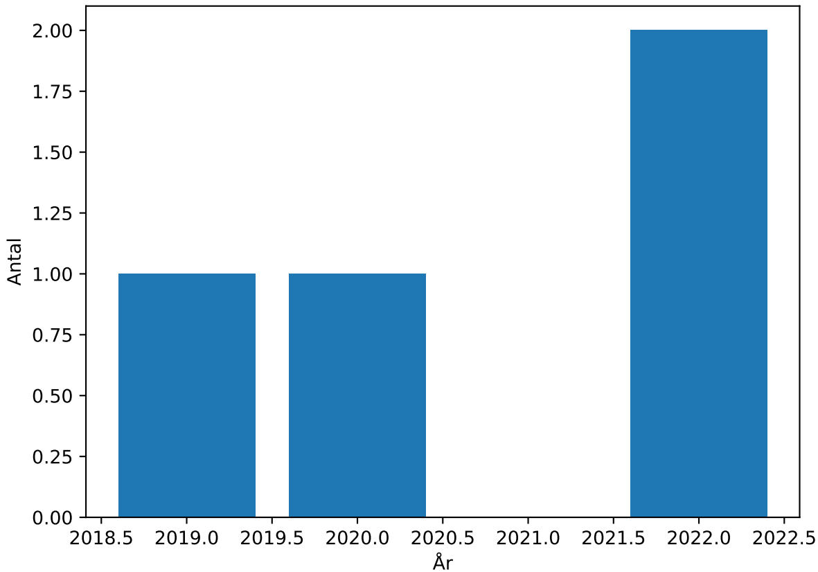
Observations per year — Gronsabbvinge
