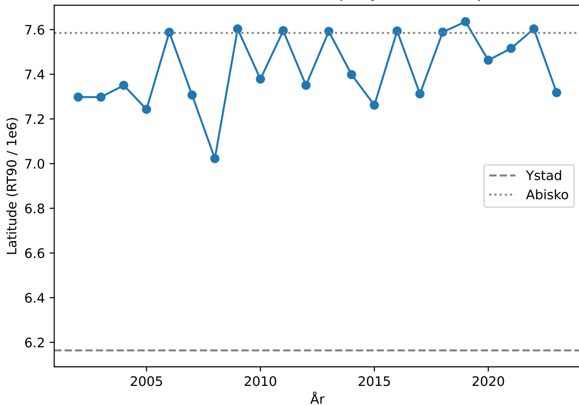
Northernmost observation per year — Tistelfjäril
