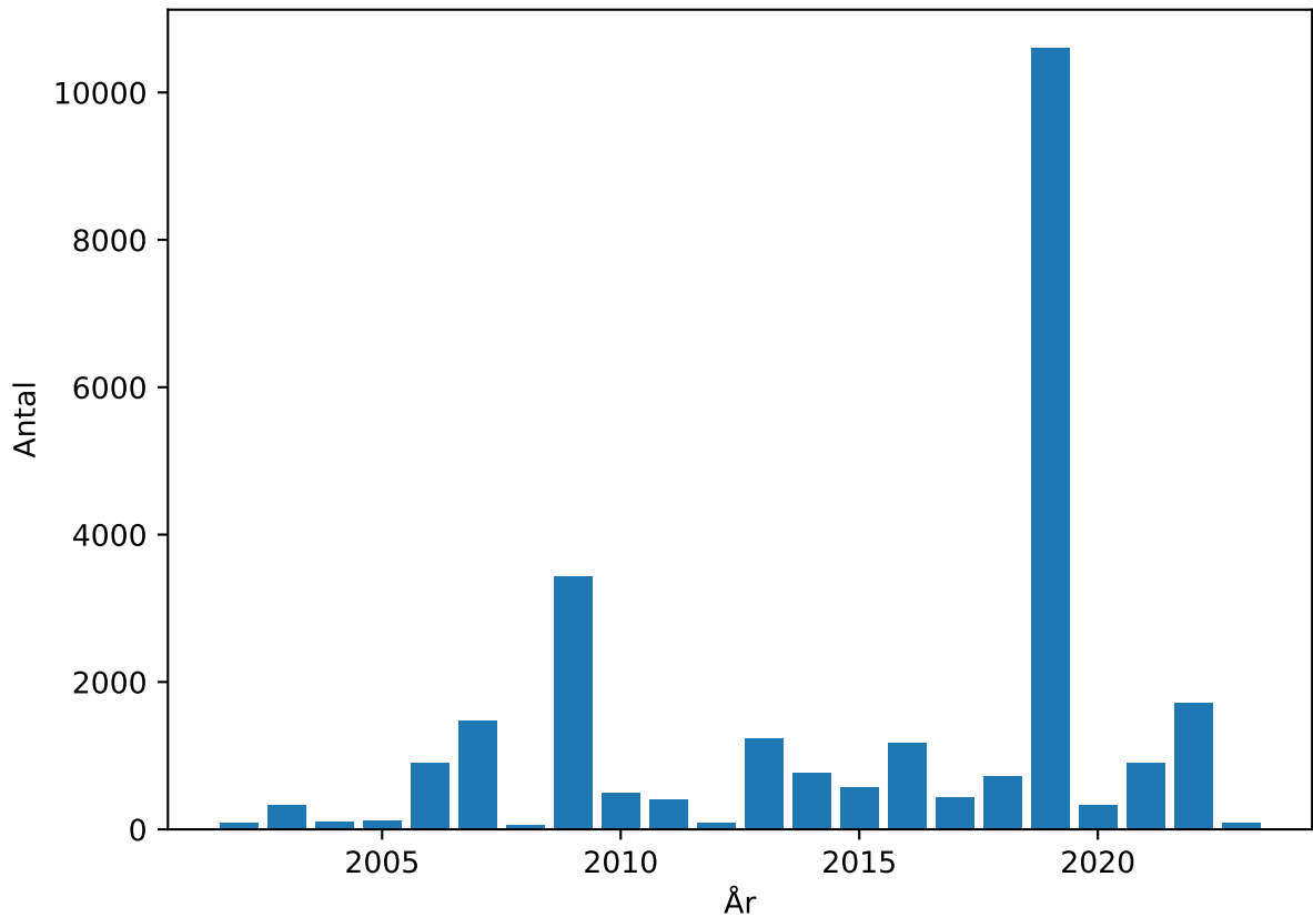
Observations per year — Tistelfjäril
