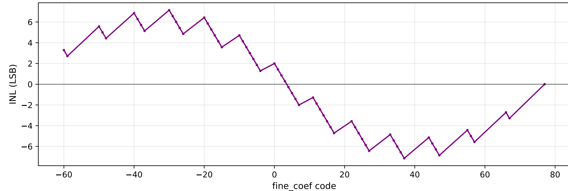
INL (worst case: +7.14 / -7.14 LSB)
