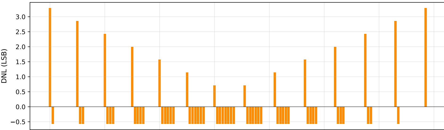
DNL (worst case: +3.29 / -0.57 LSB)
