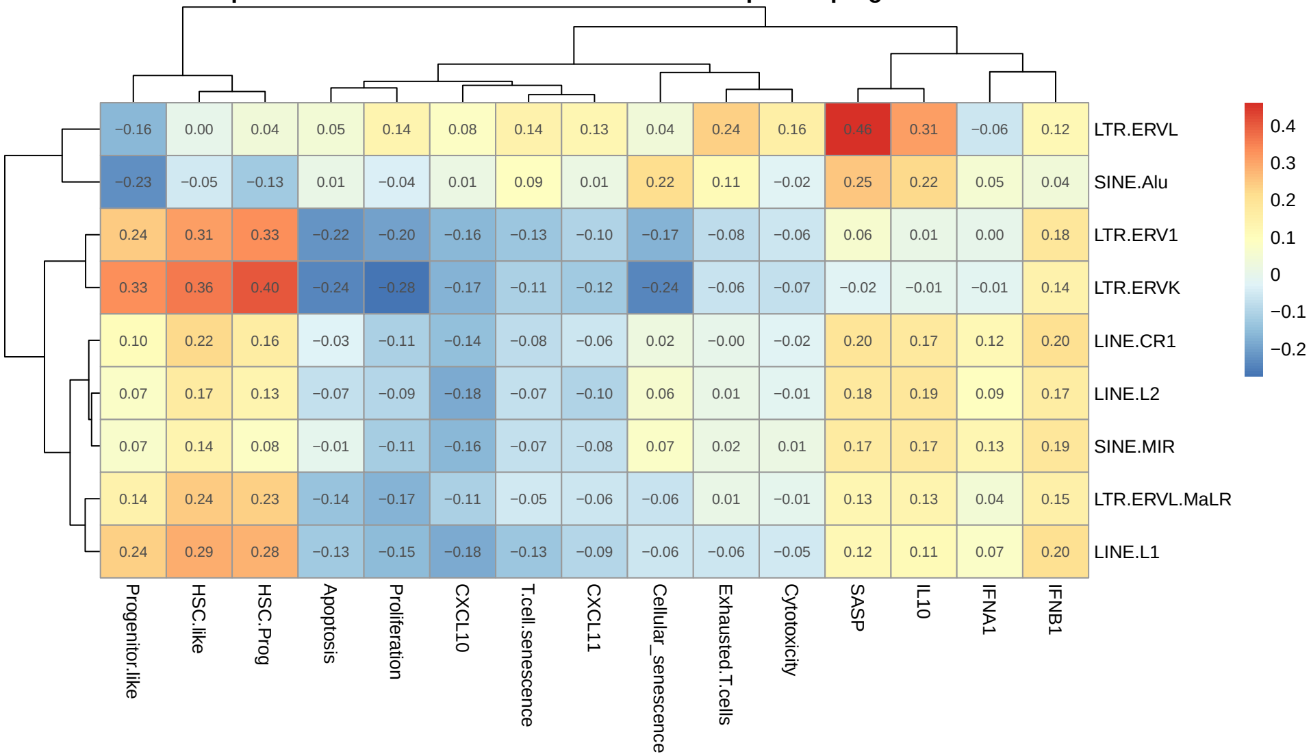
Spearman correlation: RTE features vs transcriptomic programmes
