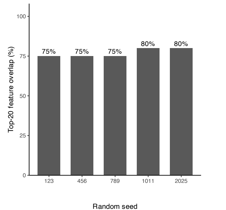
Training-validation overlap of top-20 SHAP features
