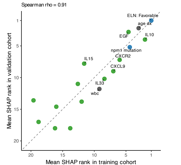
Concordance of SHAP rankings between cohorts
