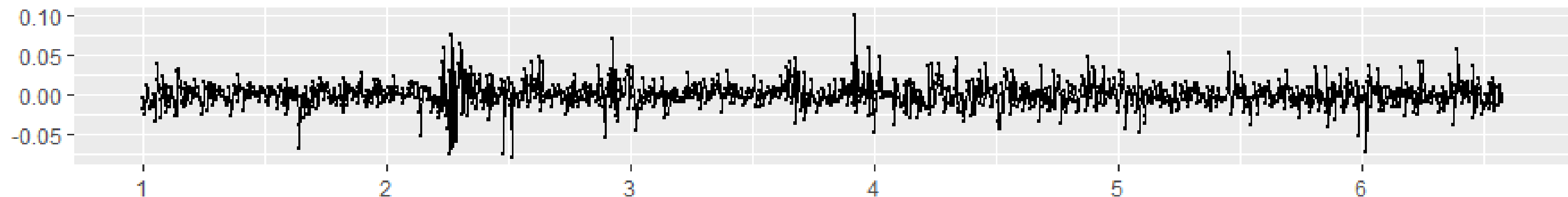
Residuals from ARIMA(1,0,3) with zero mean
