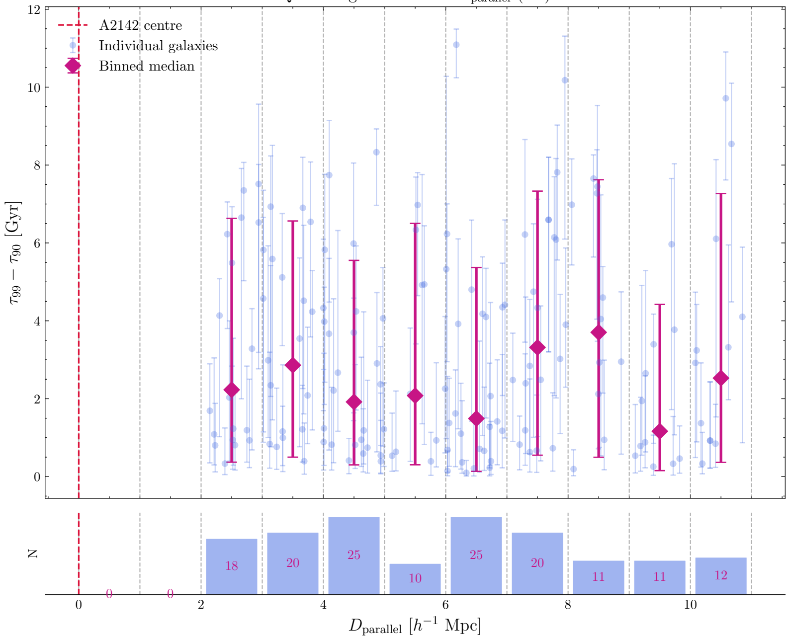
Quenching timescale vs D_{\text{parallel}} (2D)
