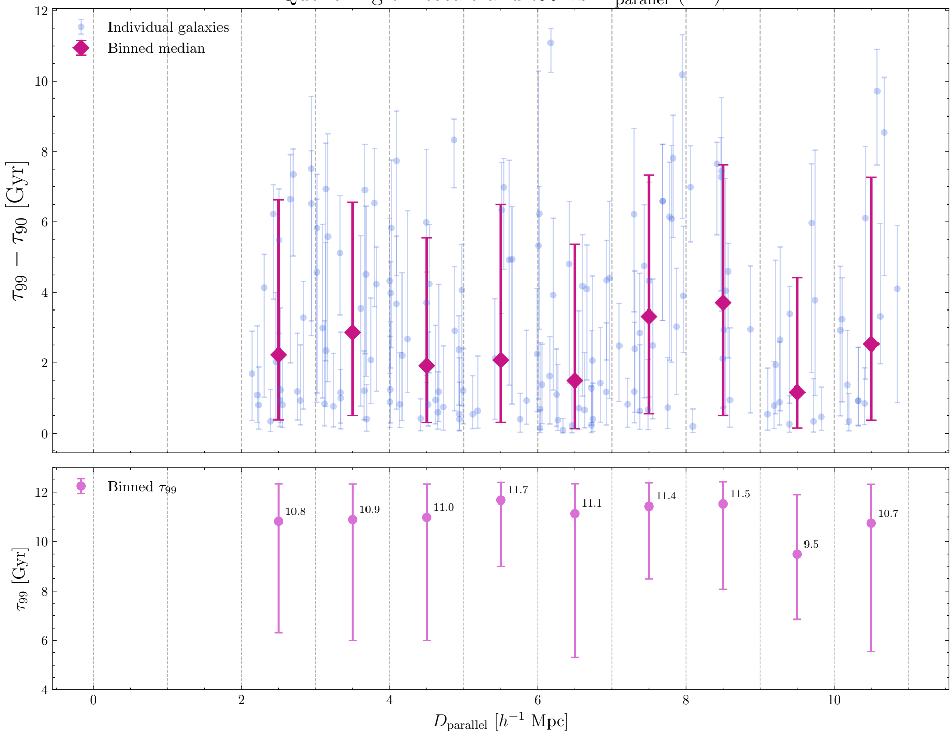
Quenching timescale and t_{99} vs D_{\text{parallel}} (2D)
