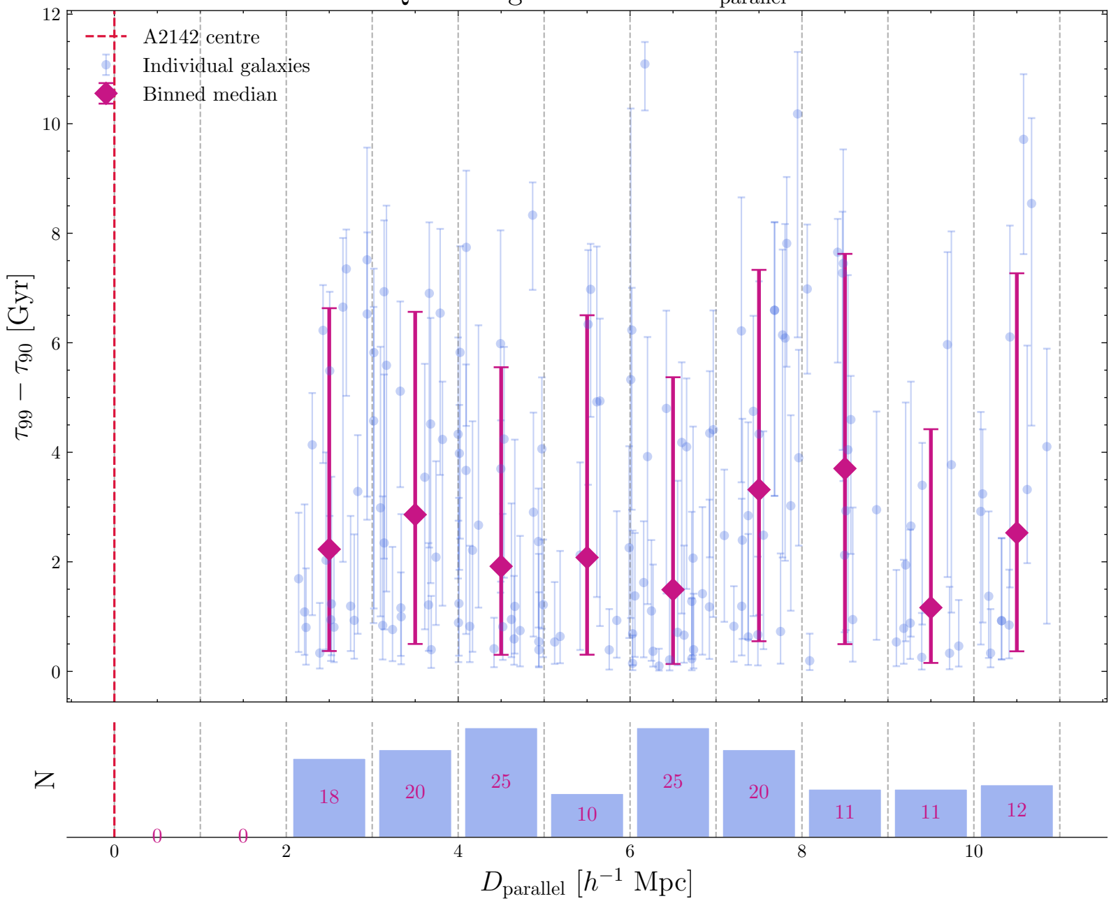
Quenching timescale vs D_{\text{parallel}}
