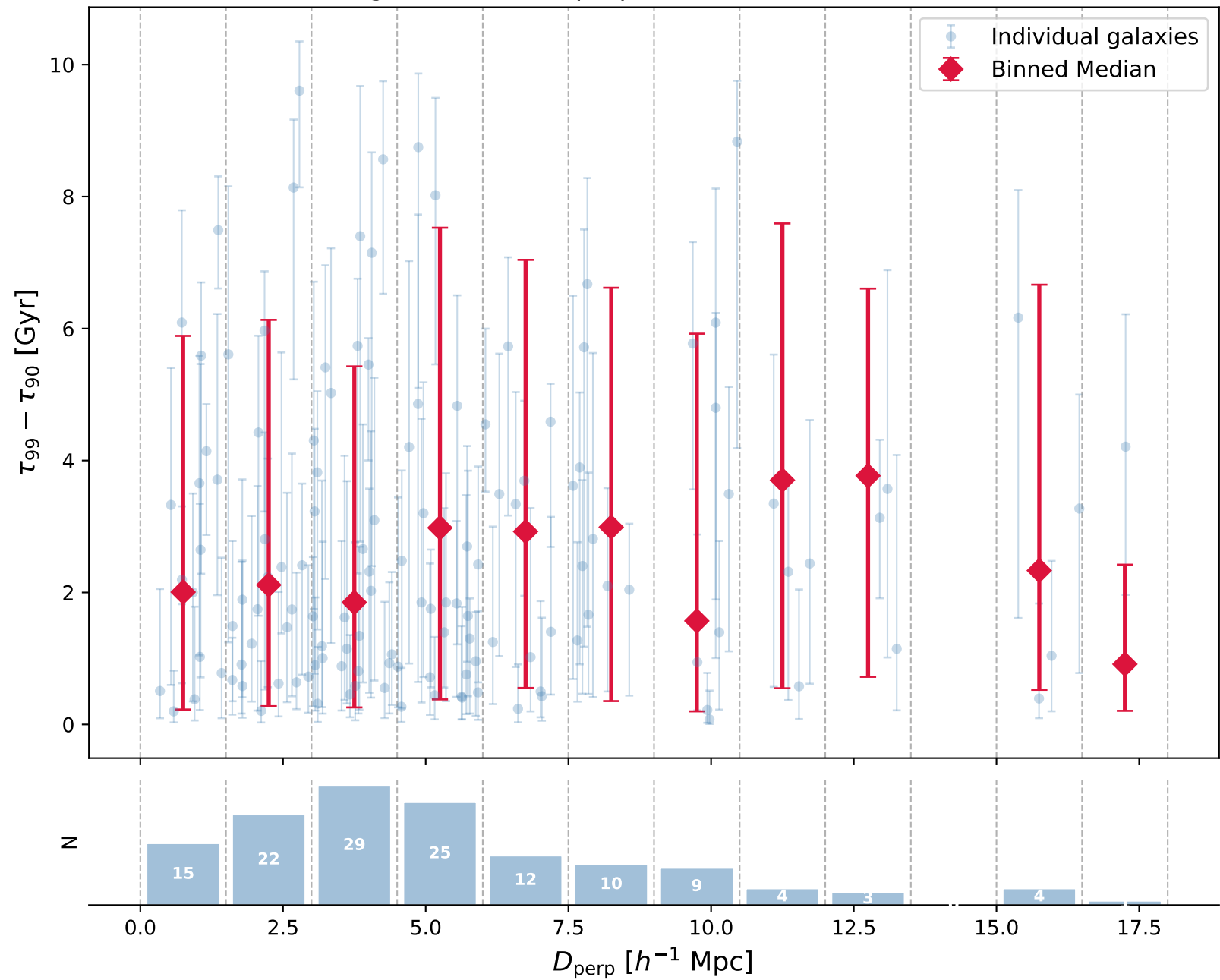
Quenching timescale vs. perpendicular distance from filament
