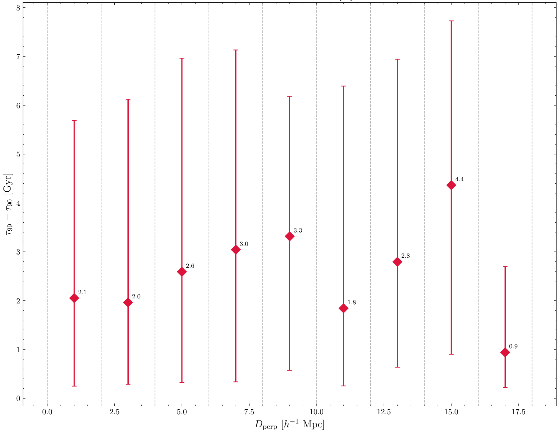
Quenching timescale vs D_{\text{perp}}
