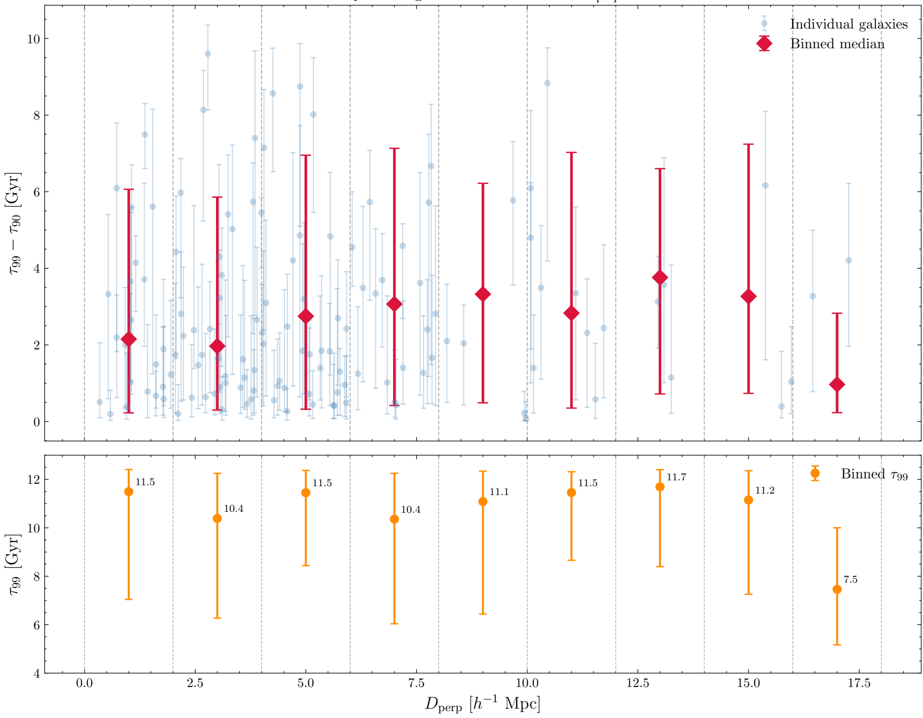
Quenching timescale and t_{99} vs D_{\text{perp}}
