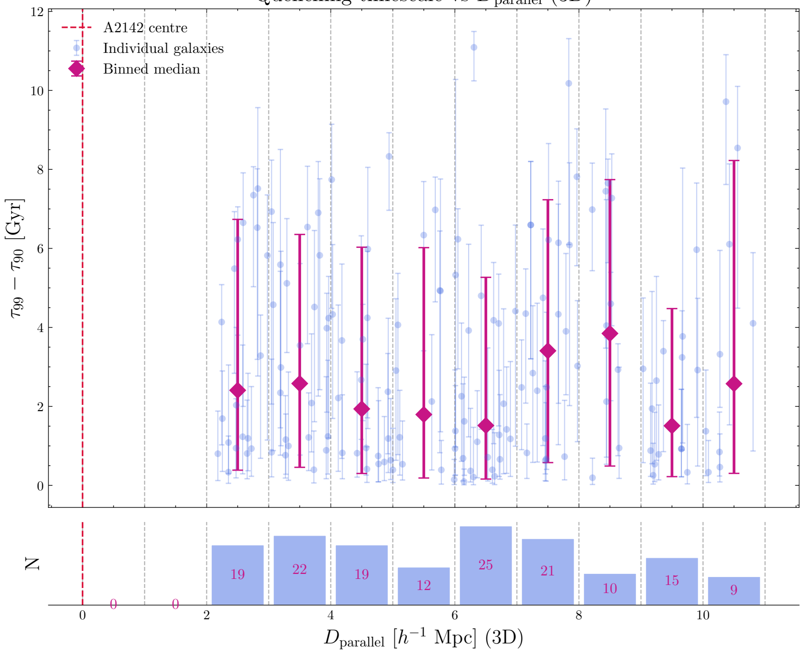
Quenching timescale vs D_{\text{parallel}} (3D)
