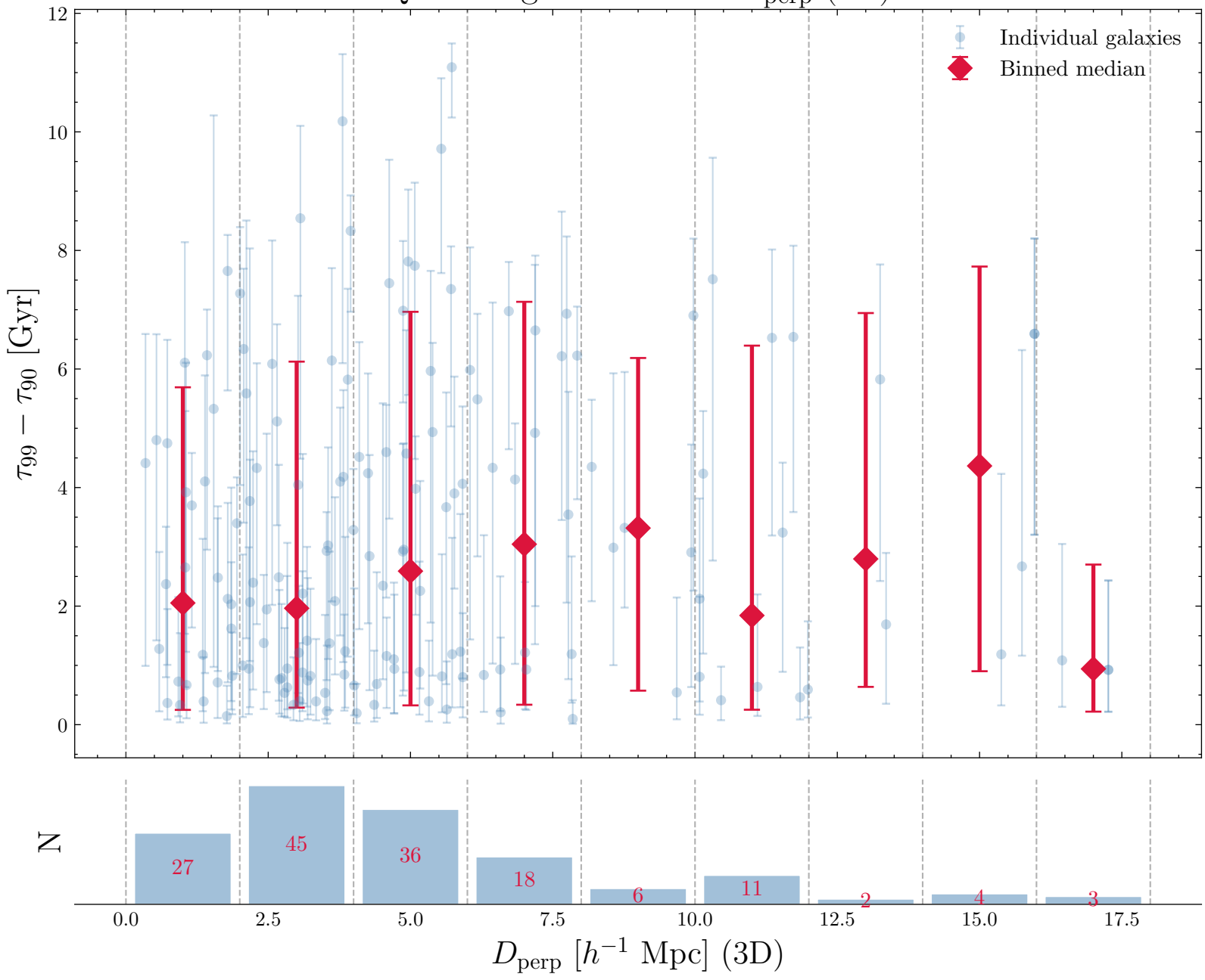
Quenching timescale vs D_{\text{perp}} (3D)
