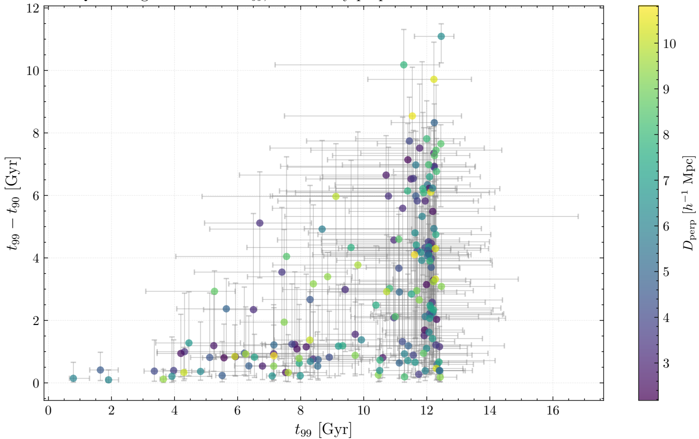
Quenching timescale vs. t_{99} , coloured by perpendicular filament distance
