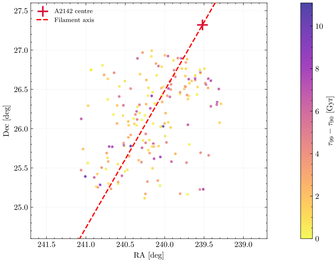
RA vs Dec
