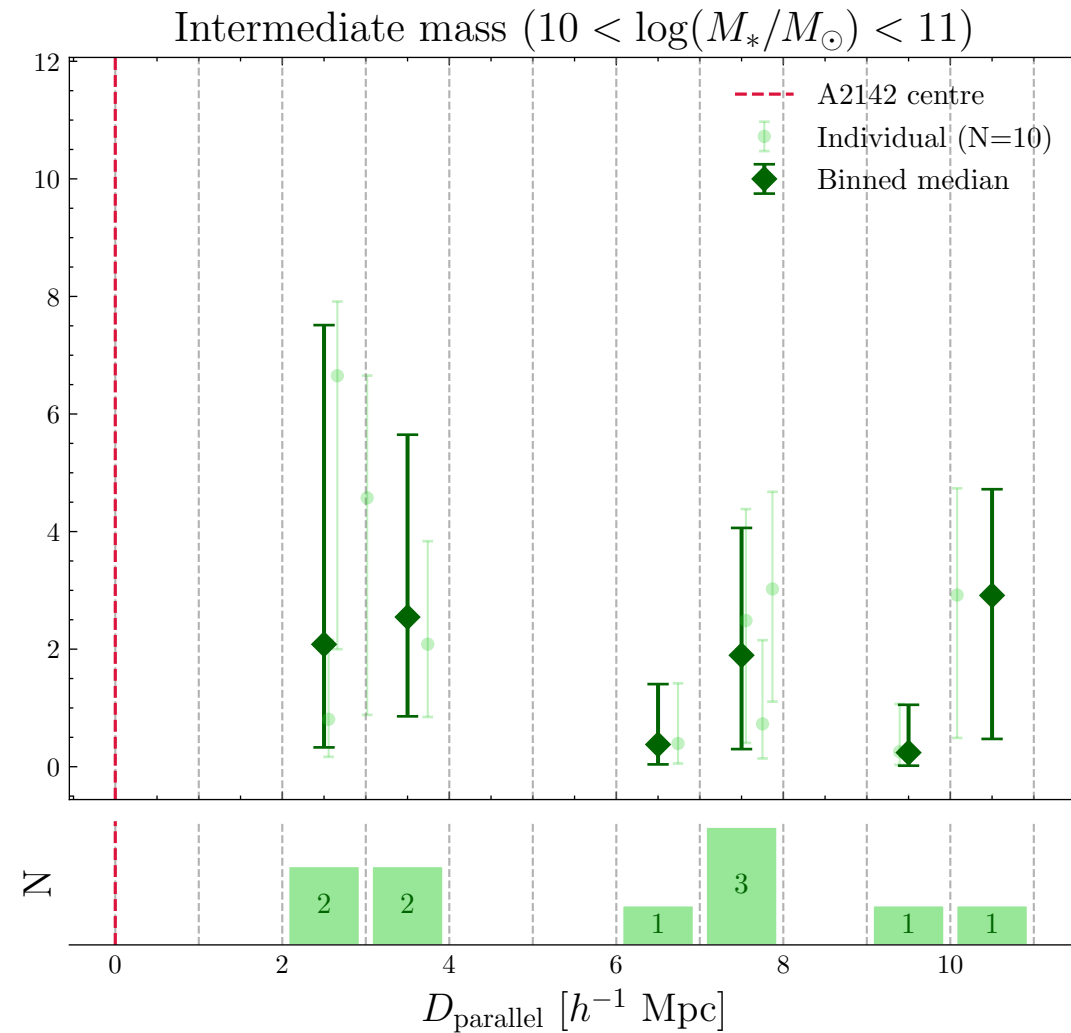
Quenching timescale vs D_{\text{parallel}} by stellar mass
