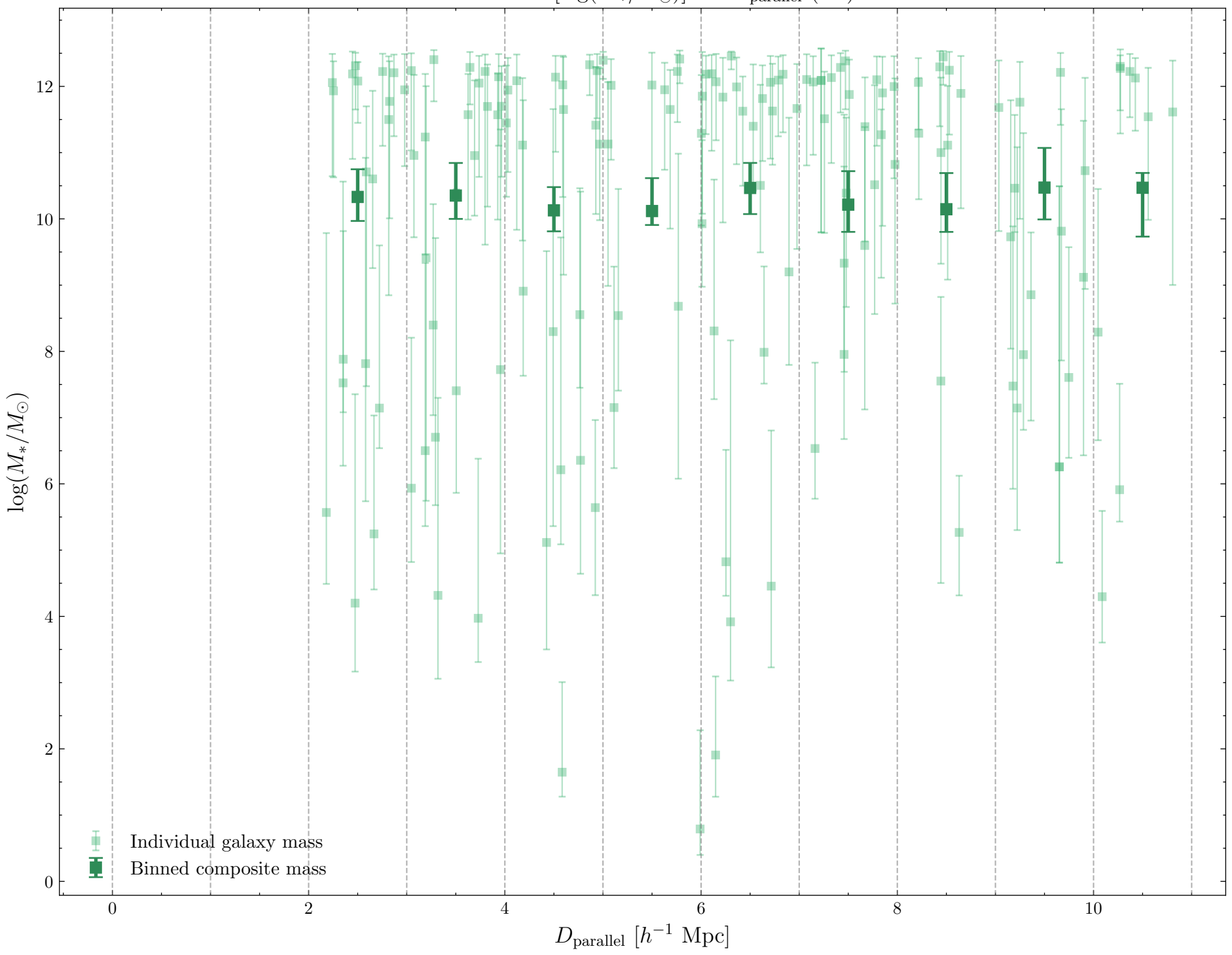
Stellar mass [ \log(M_*/M_\odot) ] vs. D_{\text{parallel}} (3D)
