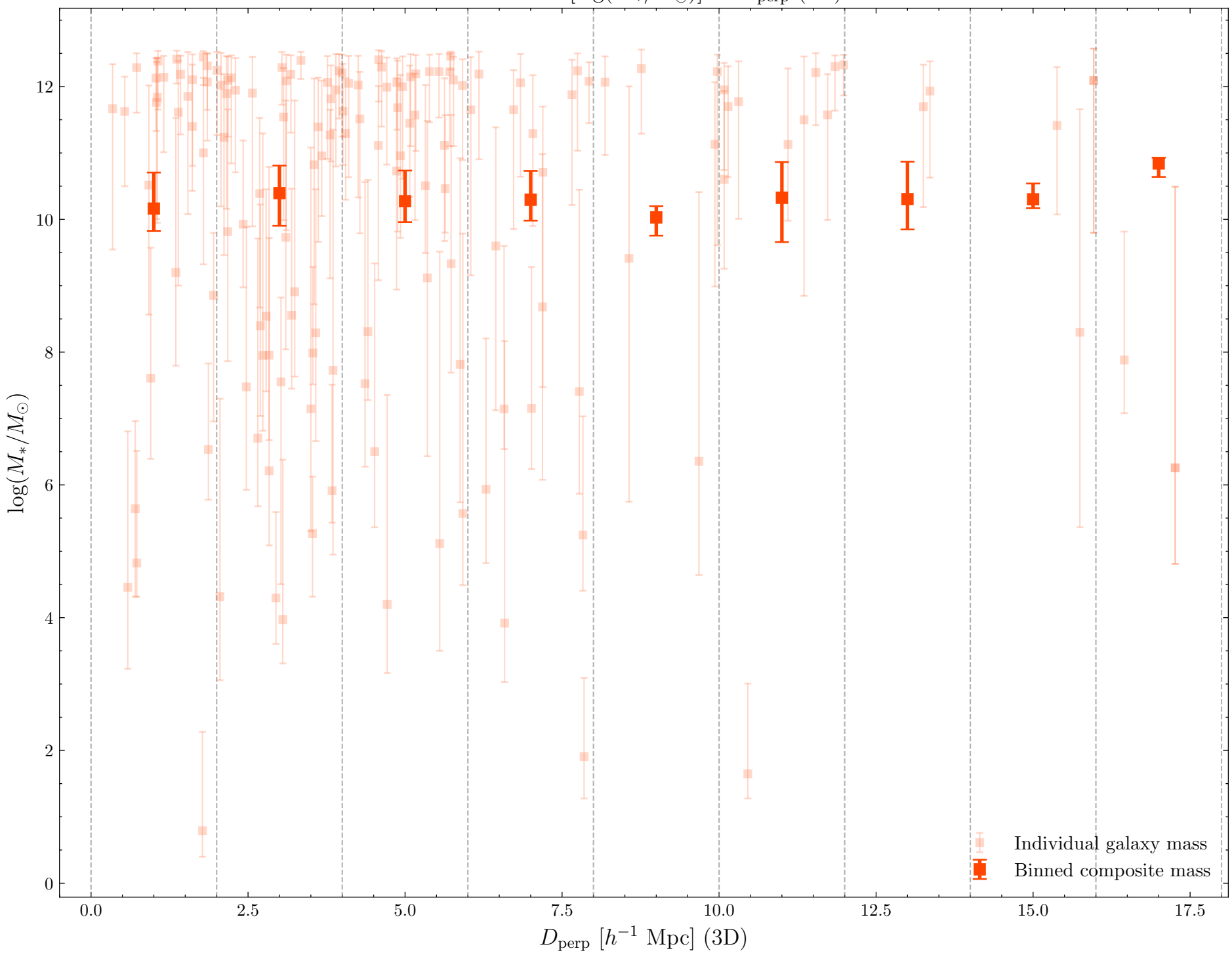
Stellar mass [ \log(M_*/M_\odot) ] vs D_{\text{perp}} (3D)
