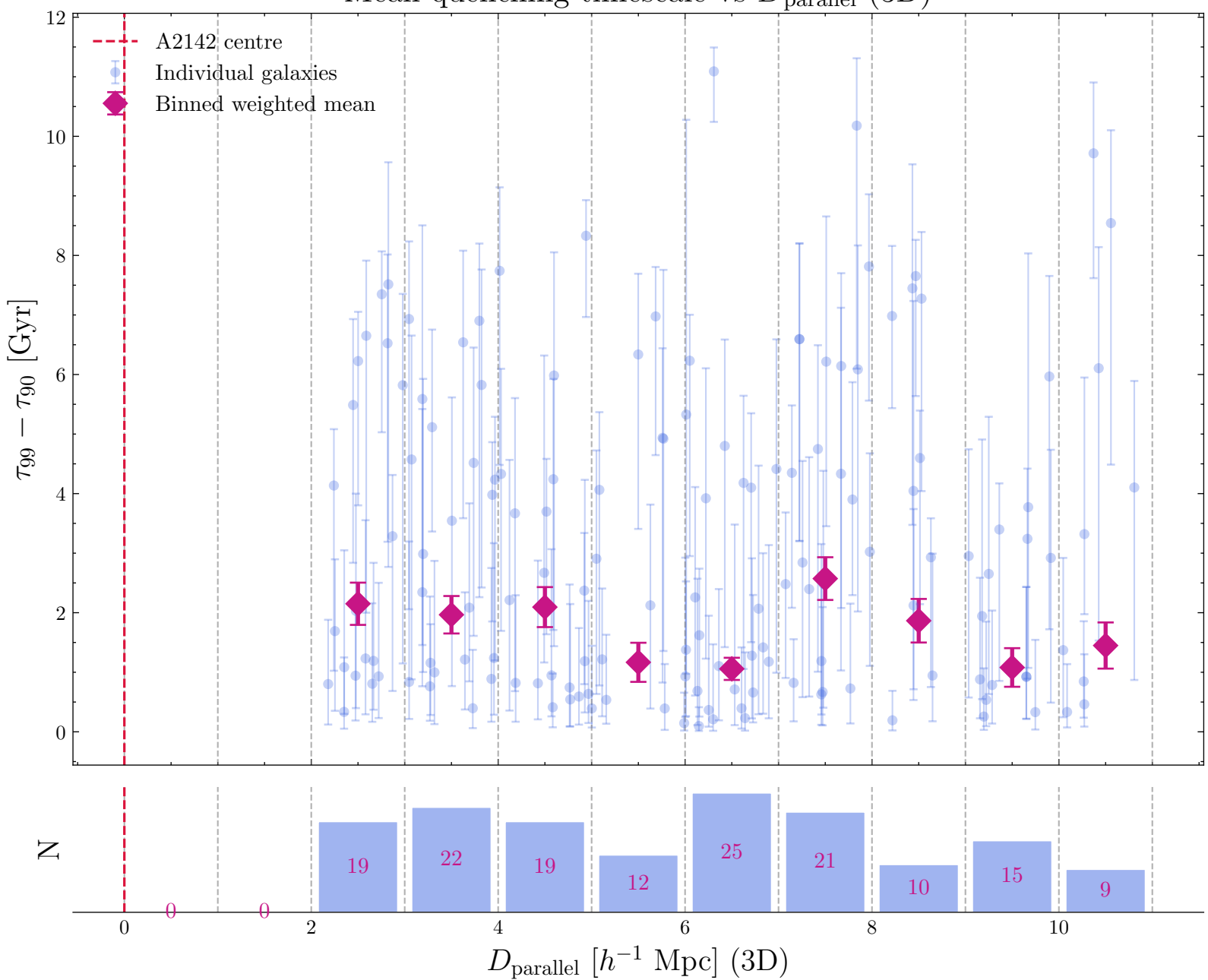
Mean quenching timescale vs D_{\text{parallel}} (3D)
