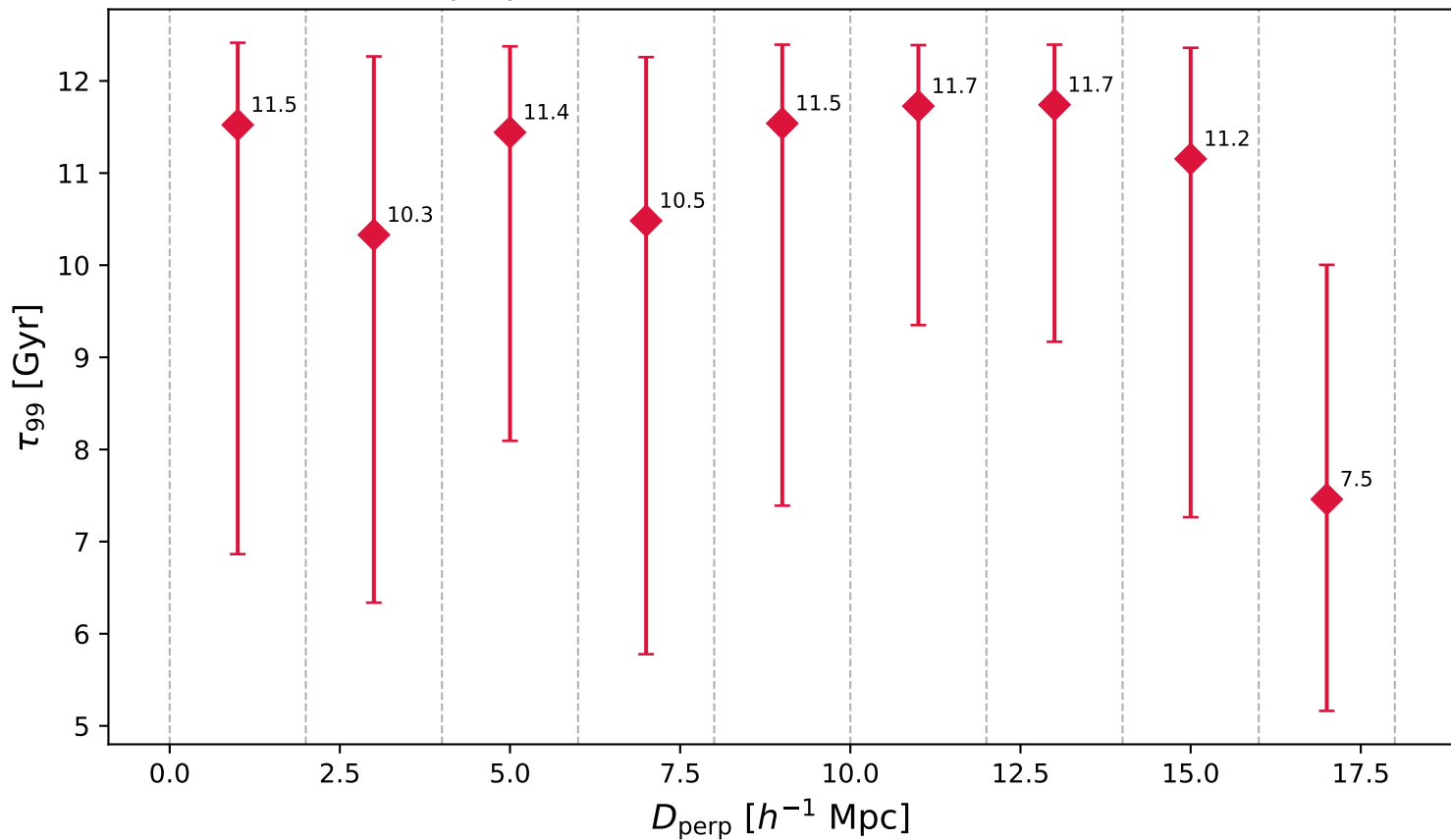
\tau_{99} vs. perpendicular distance from filament (binned)
