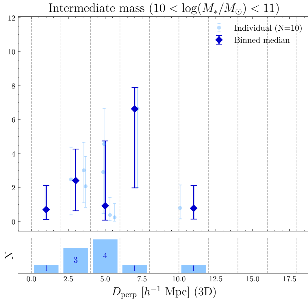
Quenching timescale vs D_{\text{perp}} (3D) by stellar mass
