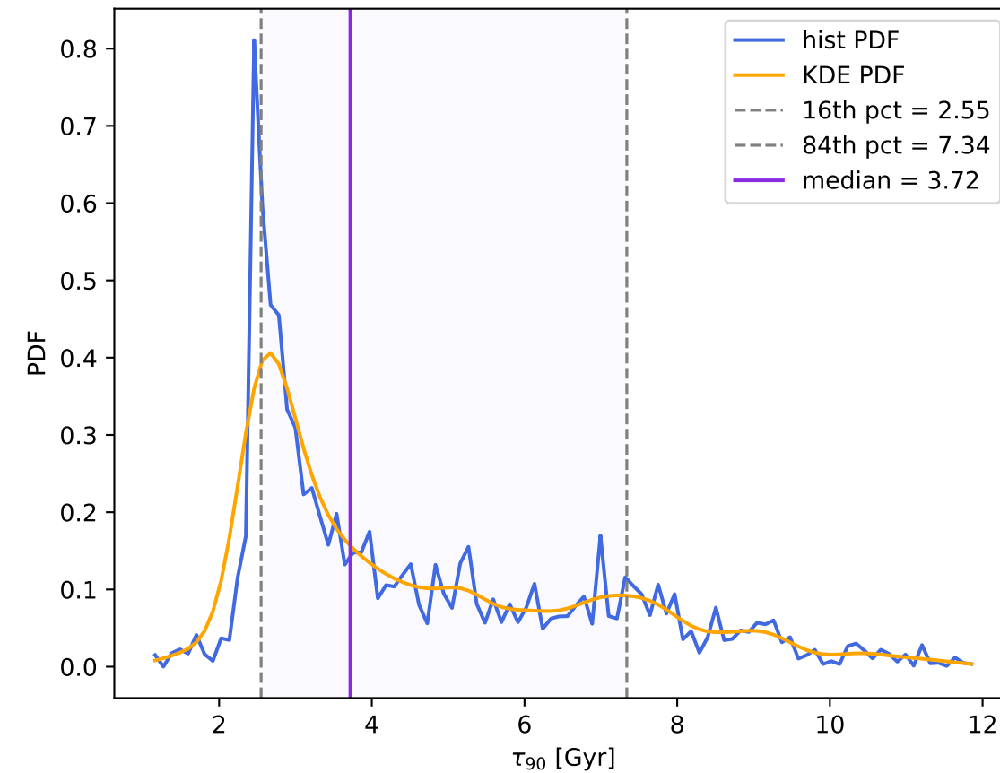
\tau_{90} Probability Density Function
