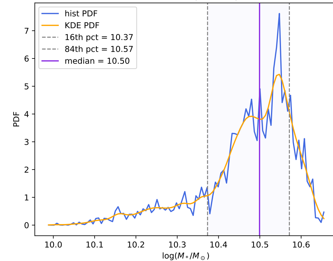
Stellar Mass Probability Density Function
