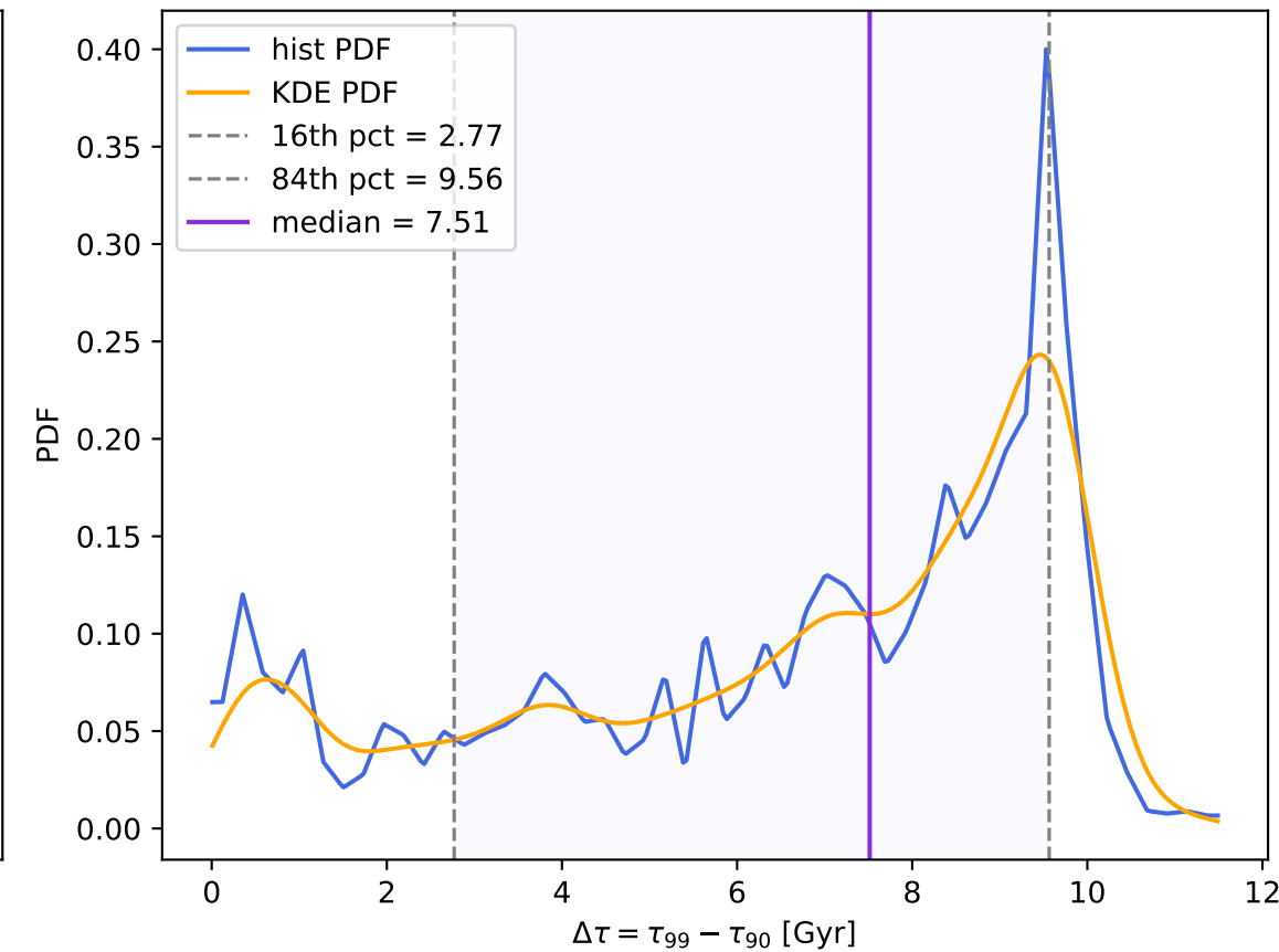
\Delta\tau Probability Density Function
