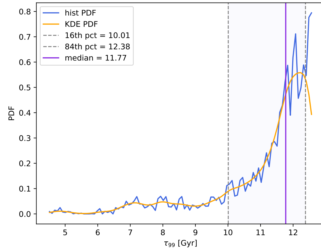
\tau_{99} Probability Density Function
