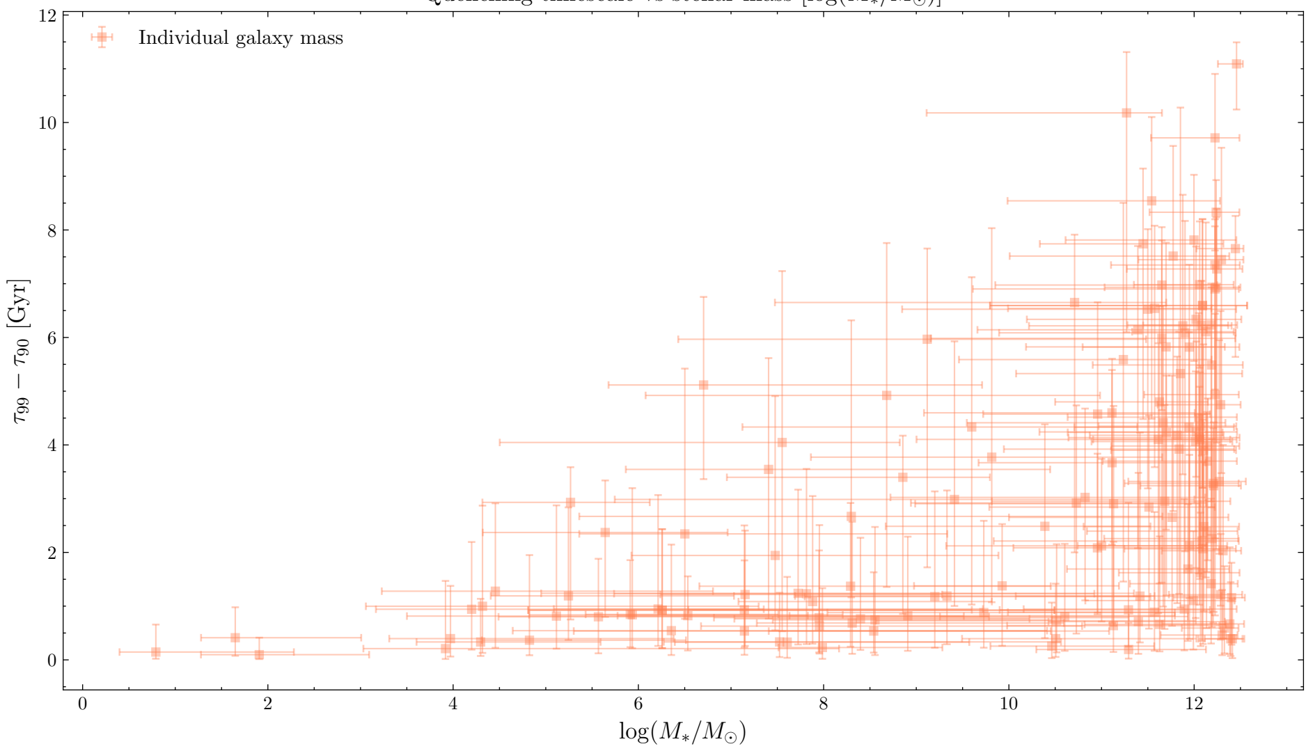
Quenching timescale vs stellar mass [ \log(M_*/M_\odot) ]
