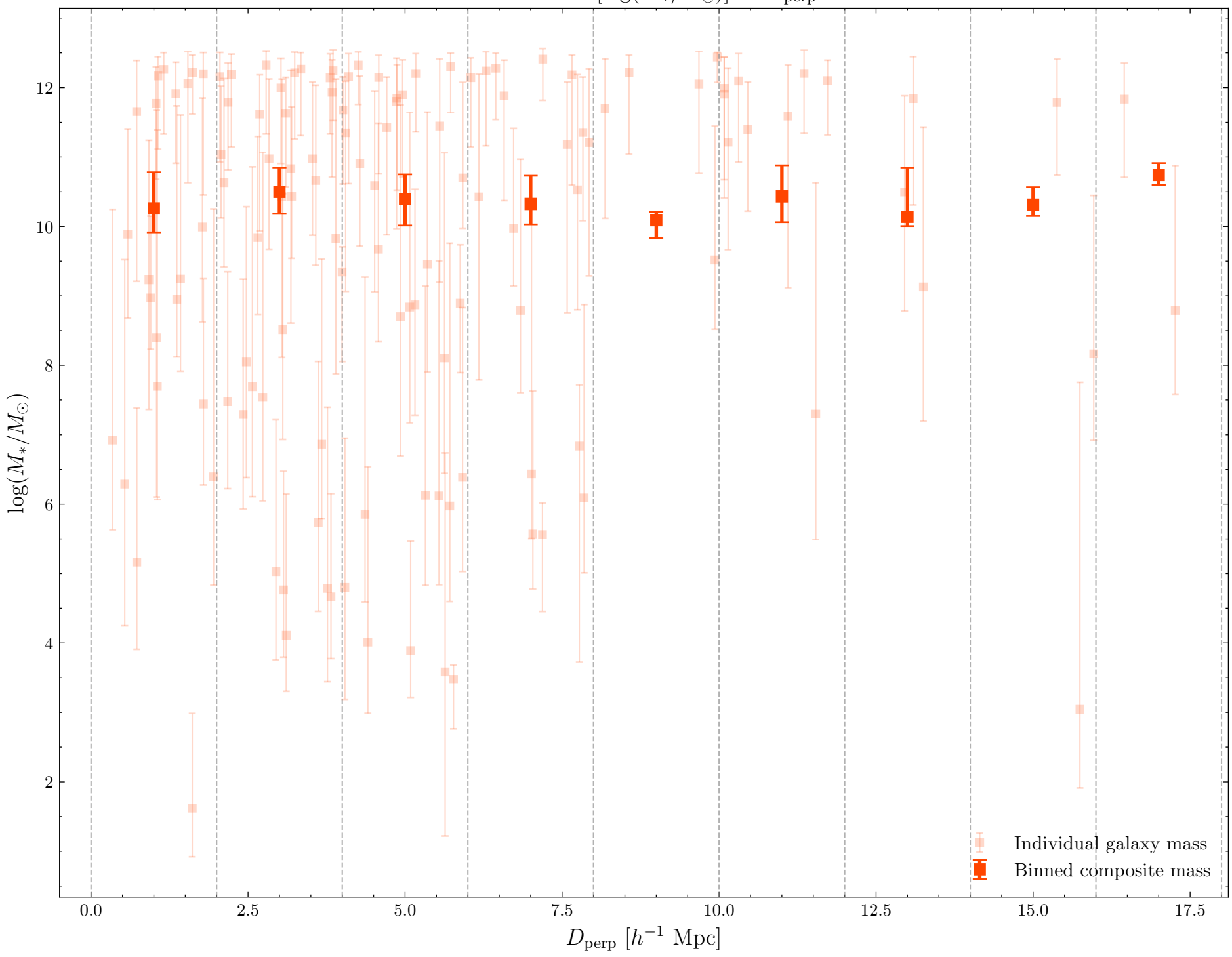
Stellar mass [ \log(M_*/M_\odot) ] vs D_{\text{perp}}
