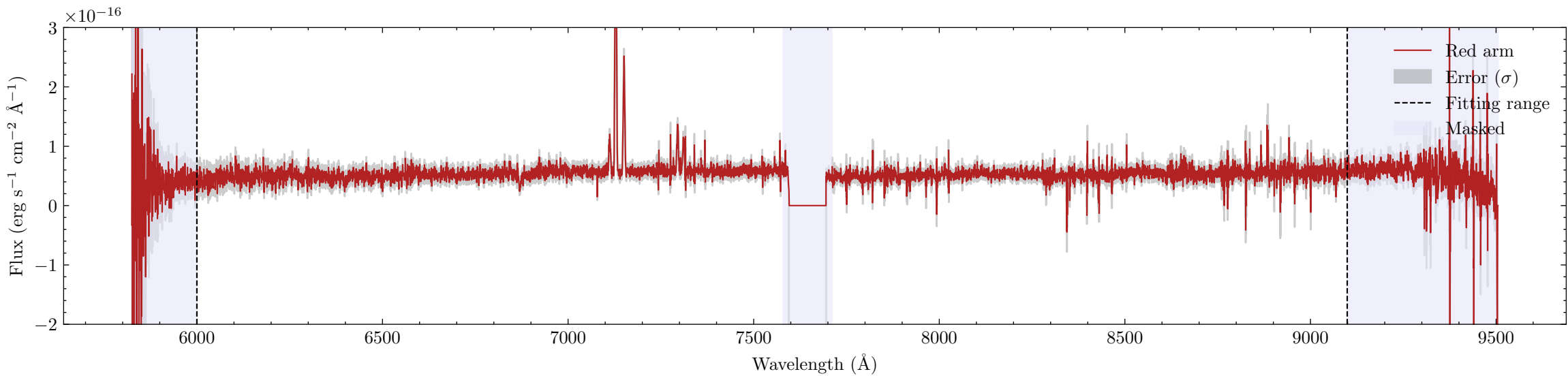
Spectra for A2142-7614, nspec=8
