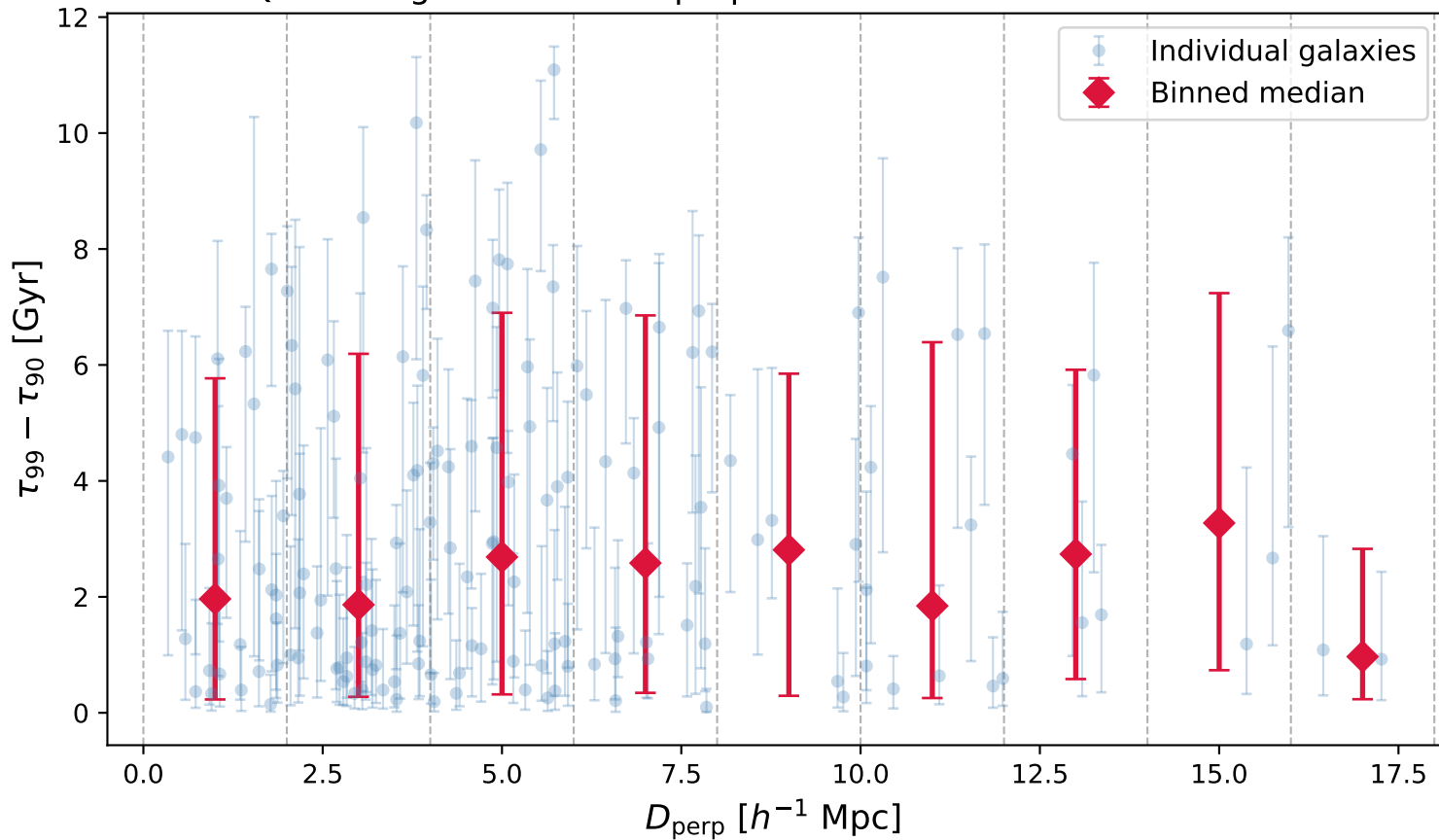
Quenching timescale vs. perpendicular distance from filament
