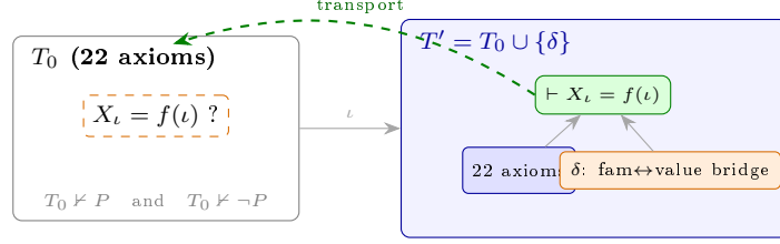
Figure 3: The move that only a theory-as-data substrate permits. How to read: each large rounded rectangle is a theory (left, the reference T_0 ; right, its extension T' ); inside, blue boxes are axioms, the orange box the added definition \delta (and, at left, the orange hypothesis it answers), the green box the goal now provable; the dashed green arrow is the transport of the result back into T_0 's language. When a hypothesis is independent (here the family-value bridge, independent of A_{T_0} ), no search closes it — the only legal move extends the theory with a definition \delta , proves the image, and transports the result back.
