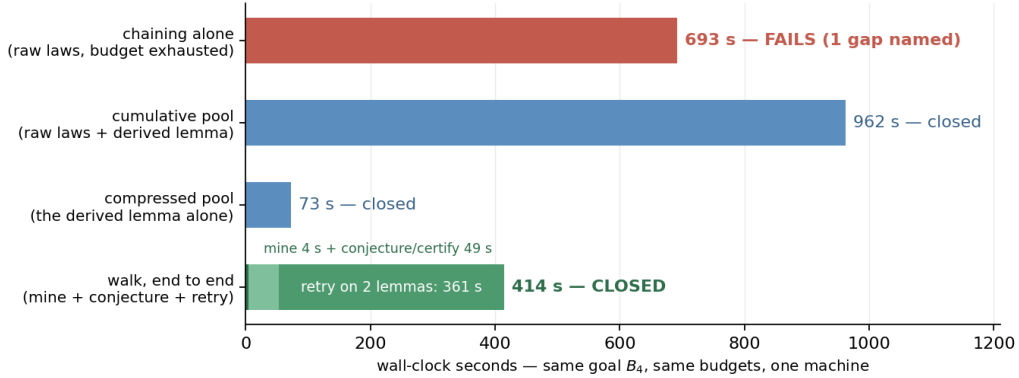
Figure 1: Four searches on the same goal B_4 , same budgets, one machine (script: scripts/gen_chronologie.py , figures from MESURES.md ). Chaining alone exhausts its budget and fails; the walk closes, and most of its time is the final retry — on the head pattern’s two lemmas only. The figure proves no generality: one goal, one bench, and failure durations depend on the measured budget caps.
