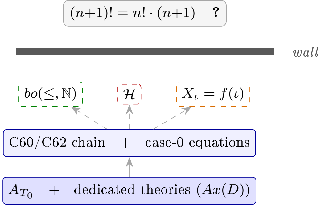
Figure 1: A real wall: the factorial front’s last open equation. Solid boxes are kernel objects, dashed boxes are the hypotheses the derivation chain leaves open , and the bar is the wall standing between them and the goal. Box colour is the trichotomy verdict of Table 1.
