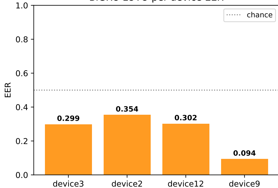
BiGRU LOTO per-device EER
