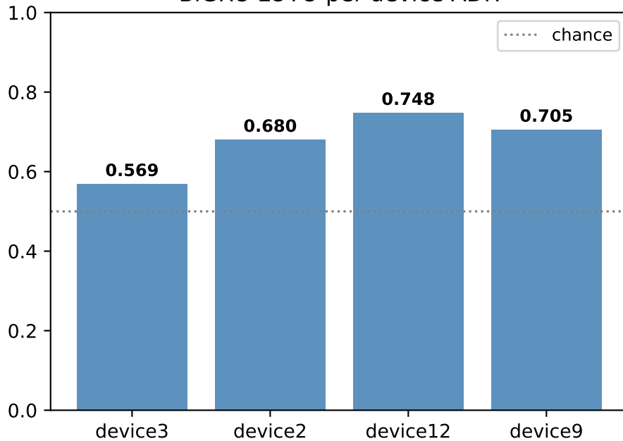
BiGRU LOTO per-device ADR
