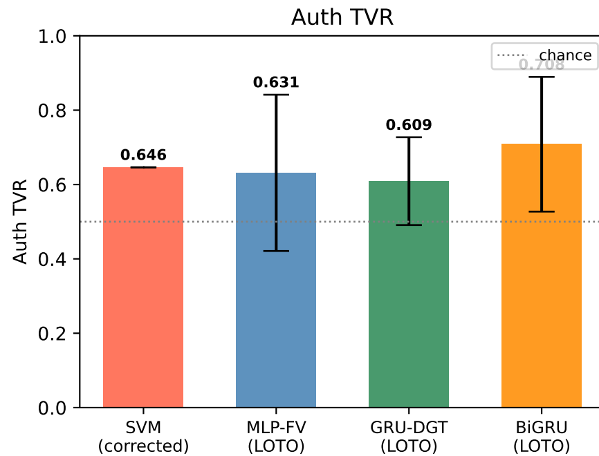
ML vs DL (LOTO) — trial_1 (SVM: 1 run; DL error bars: per-device std)
