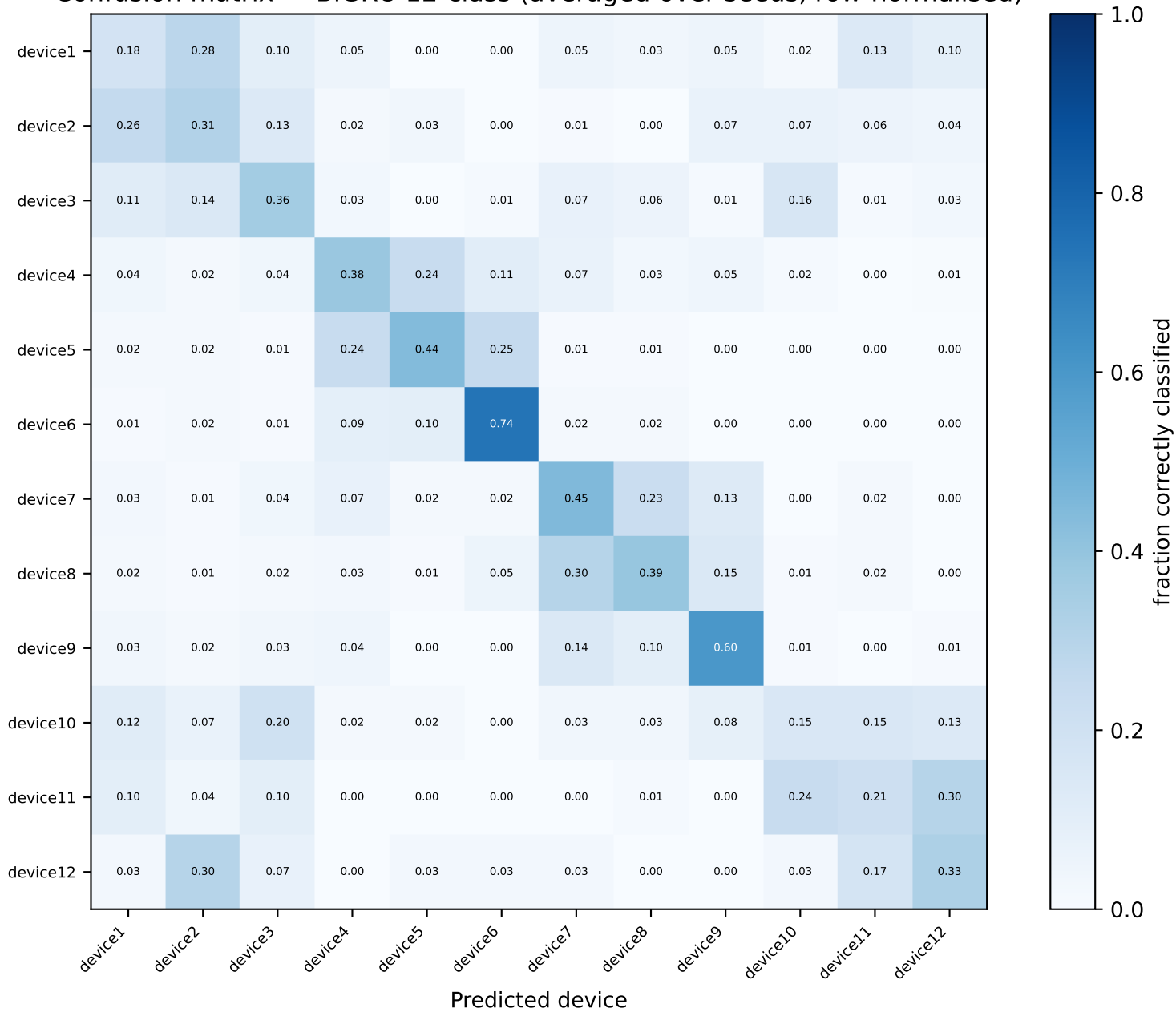
Confusion matrix — BiGRU 12-class (averaged over seeds, row-normalised)
