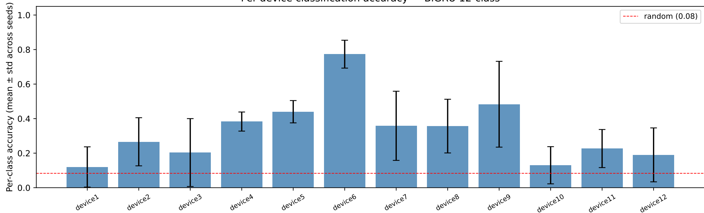
Per-device classification accuracy — BiGRU 12-class
