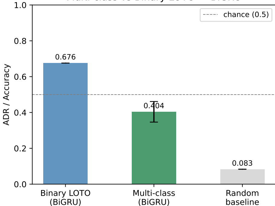
Multi-class vs Binary LOTO — BiGRU
