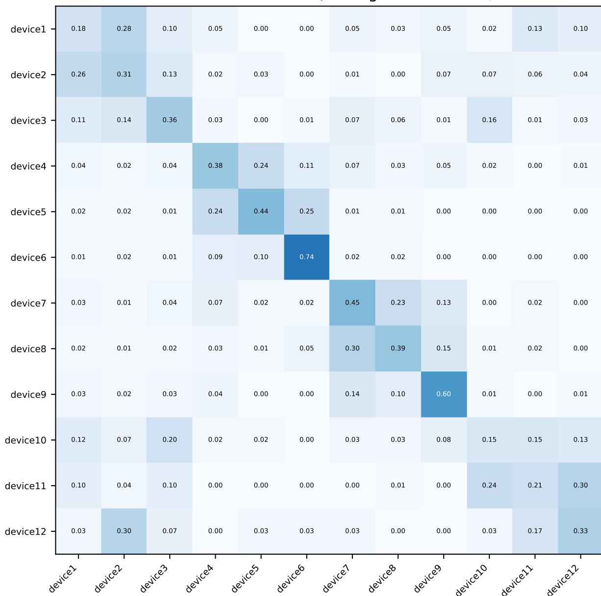
Confusion matrix — BiGRU 12-class (averaged over seeds, row-normalised)
