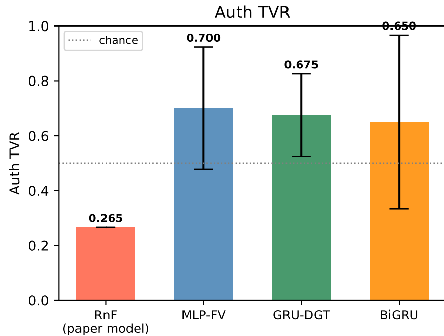
ML vs DL — trial_1 (RnF: 1 run; DL: 5 seeds \pm std)
