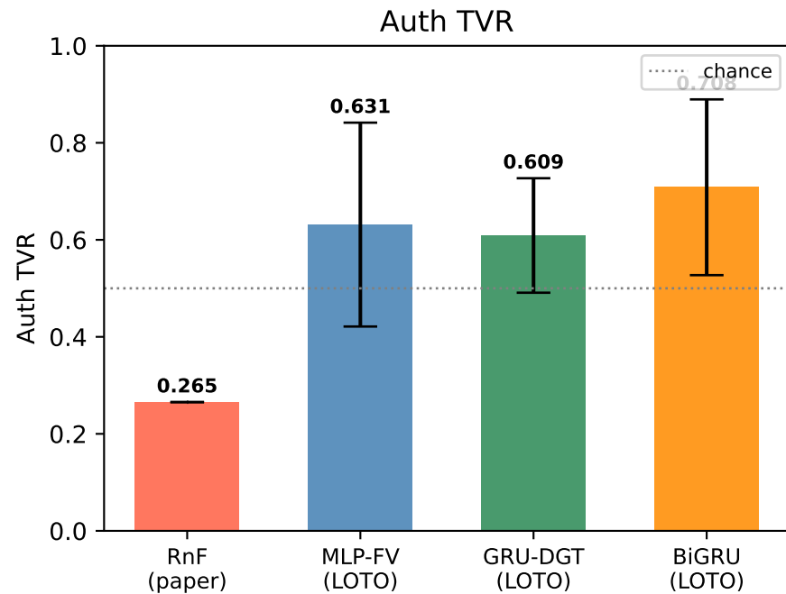
ML vs DL (LOTO) — trial_1 (RnF: 1 run; DL error bars: per-device std)
