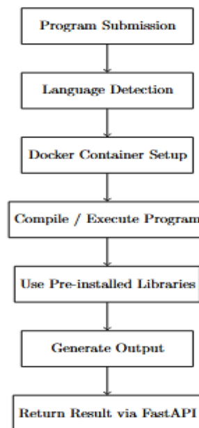
Figure 1: Simple Execution Flow of Multi-Language Compiler Backend
