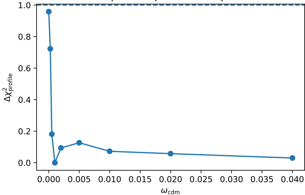
Independent particle-CDM profile
