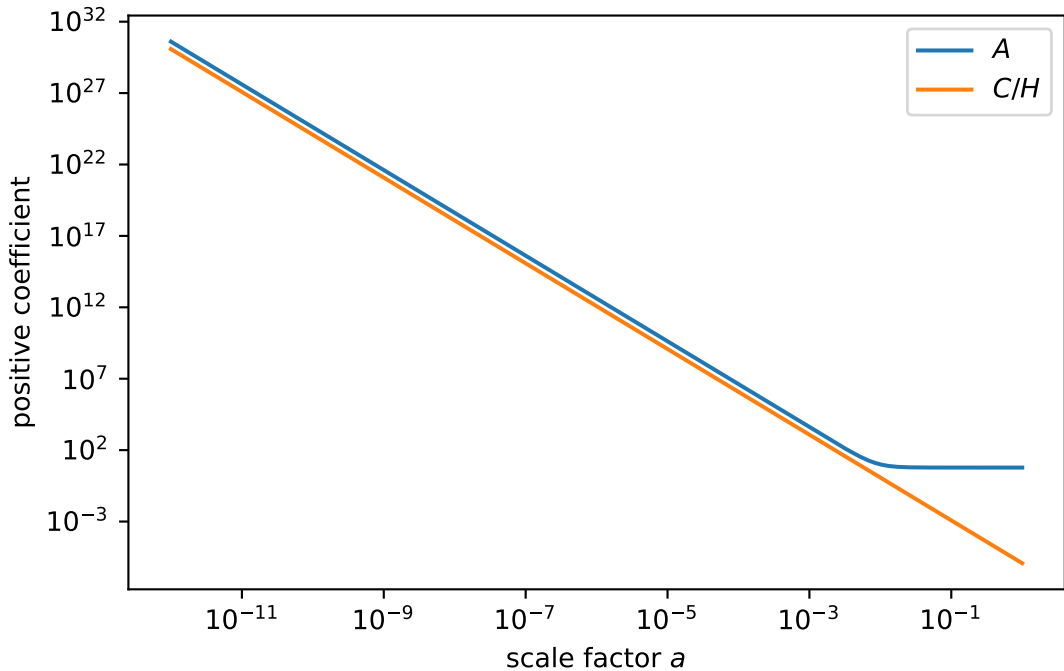
Radiation-sector Hurwitz coefficients
