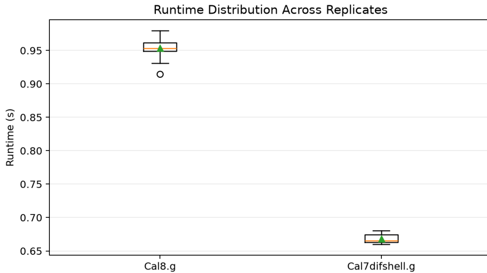
Figure 2: CPU baseline runtime distributions (boxplot). Whiskers extend to 1.5 IQR; low spread (CV \approx 1\% ) confirms stable CPU timing.
