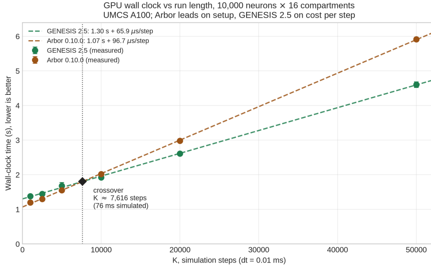
Figure 6: GPU wall clock against run length for the multi-compartment benchmark, N = 10\,000 neurons \times 16 compartments on the UMCS A100, six run lengths, mean \pm std over 3 replicates each. Both simulators are linear in K with different intercepts and slopes: Arbor starts 0.23s ahead on setup, GENESIS 2.5 advances each step 32% more cheaply. Neither is faster in general — the lines cross at K \approx 7600 , and a comparison at a single run length reports whichever side of that the author happened to choose.
