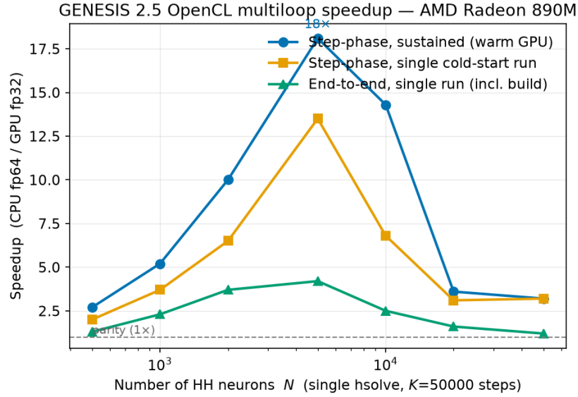
Figure 2: Measured wall-clock speedup, GPU multiloop (fp32) vs. CPU (fp64), after the scheduler and Hines-solver fixes. Step-phase speedup is shown for the GPU's sustained (warm) clock state and for a single cold-start run; the two differ because the CPU-bound model build downclocks the idle GPU before the first dispatch. Both peak near N = 5000 and fall beyond N \approx 10000 as the integrated GPU stops sustaining its fast clocks. End-to-end (single run, including construction) is lower still.
