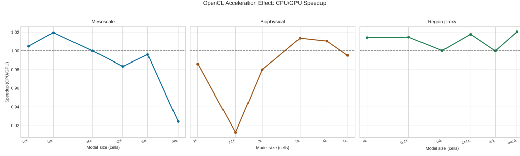
Figure 7: CPU vs. GPU end-to-end speedup ratio (per-step dispatch mode) across N . Values below 1\times indicate that per-step PCIe transfer overhead makes the GPU path slower than CPU for this N range.
