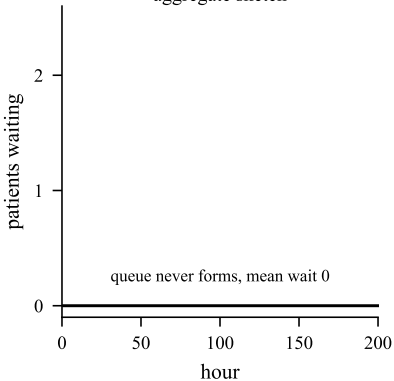
aggregate sketch
