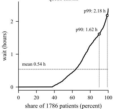
queue sketch
