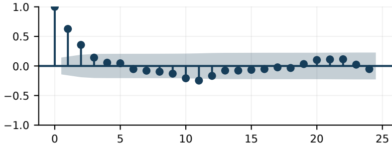
Partial Autocorrelation
