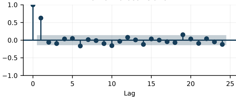
Partial Autocorrelation
