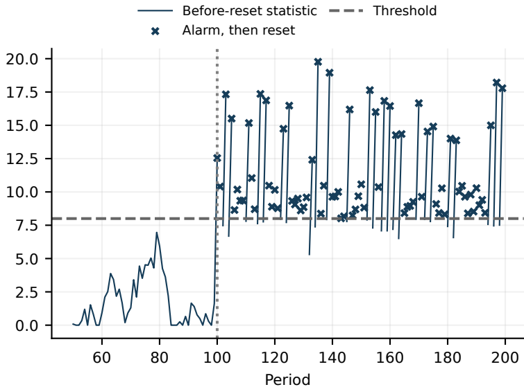
One-sided CUSUM
